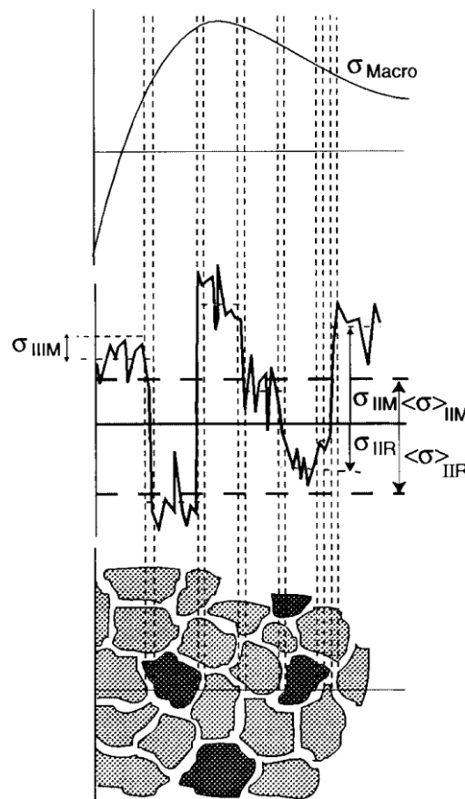
Fig. 2.11. Schematic of possible internal stresses within a material [32].
