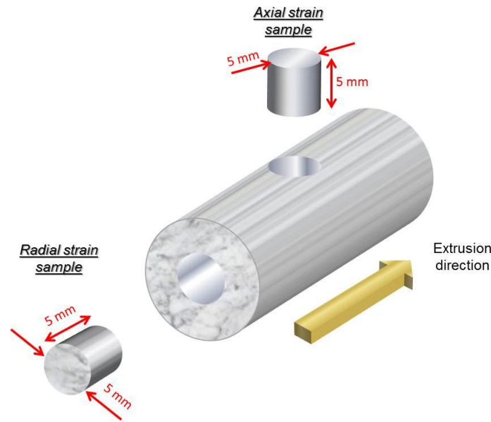
Fig. 3.12. Samples of the PM materials machined by spark erosion with length and diameter of 5 mm and axis oriented parallel (axial) and orthogonal (radial) to the extrusion direction, respectively.
