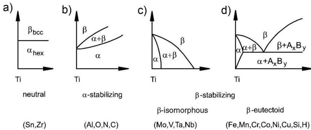
Fig. 2.6. Effect of alloying elements on phase diagrams of titanium alloys [3].
