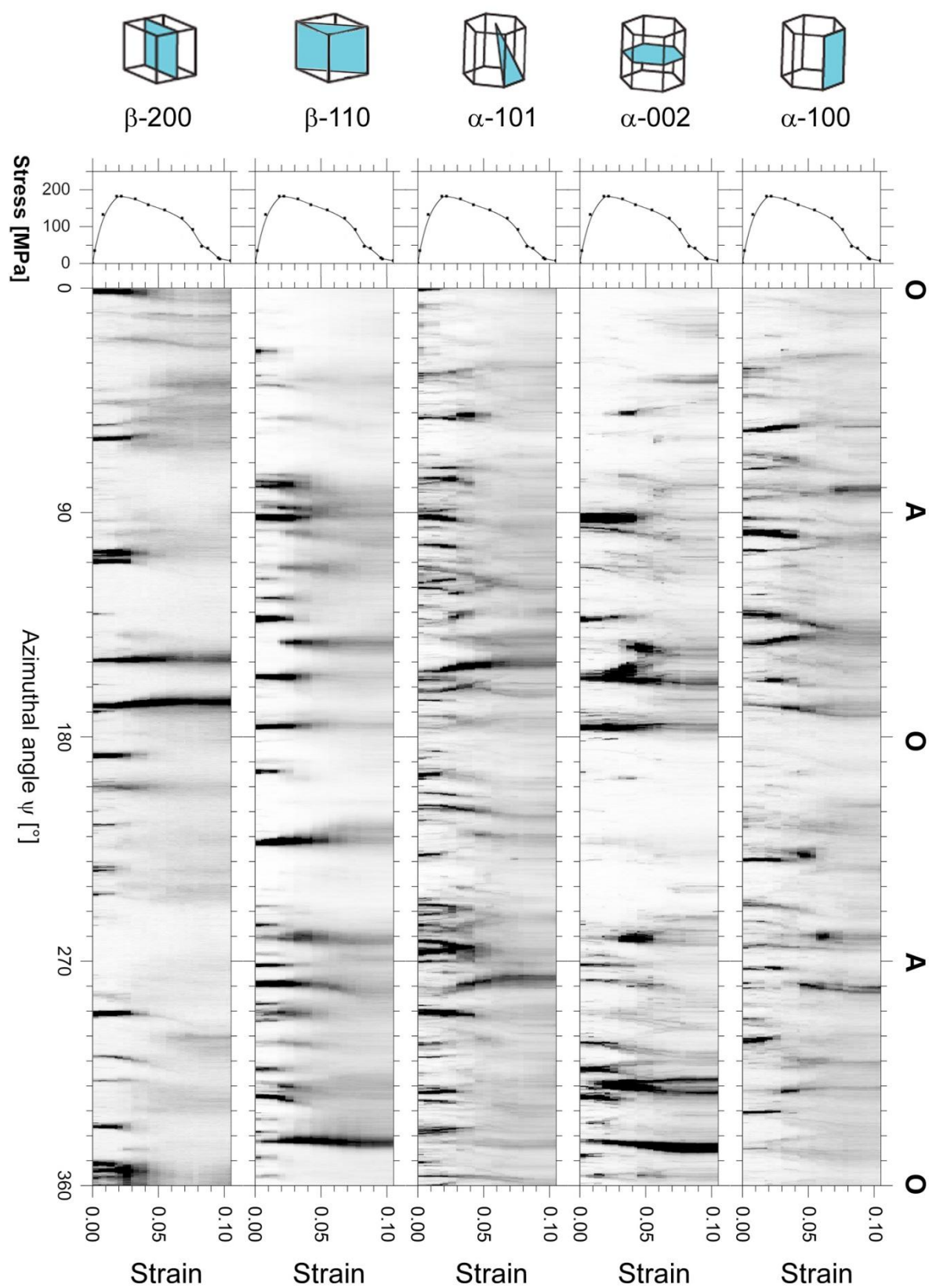
Fig. 4.16. AS-plots for three \alpha - and two \beta -reflections of the PM alloy at 750°C. The azimuthal angle is indicated at the bottom and axial (A) and orthogonal (O) directions at the top. The plot on the left side corresponds to the macroscopic stress vs. strain curve.
