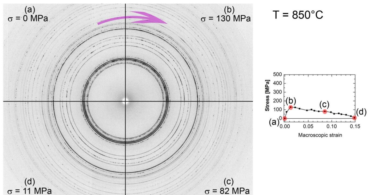
Fig. 4.33. Representative portions of the acquired diffraction rings assembled with four sectors for the Ti662/TiC/12p at 850^{\circ}\text{C} . Corresponding \alpha -, \beta - and TiC-planes are indicated in Fig. 3.24 b). On the right, the macroscopic stress vs. strain curve is plotted.
