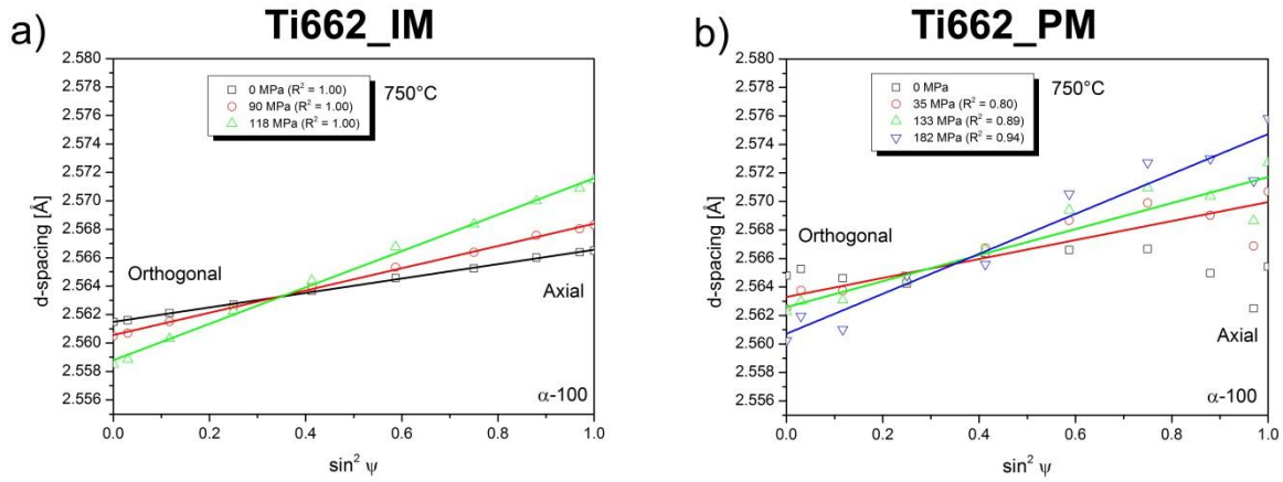
Fig. 4.8. d vs \sin^2 \psi plots with the linear fits at different stresses for the \alpha -100 Ti reflection at 750°C: a) Ti662 IM alloy b) Ti662 PM alloy. R^2 values are also indicated.
