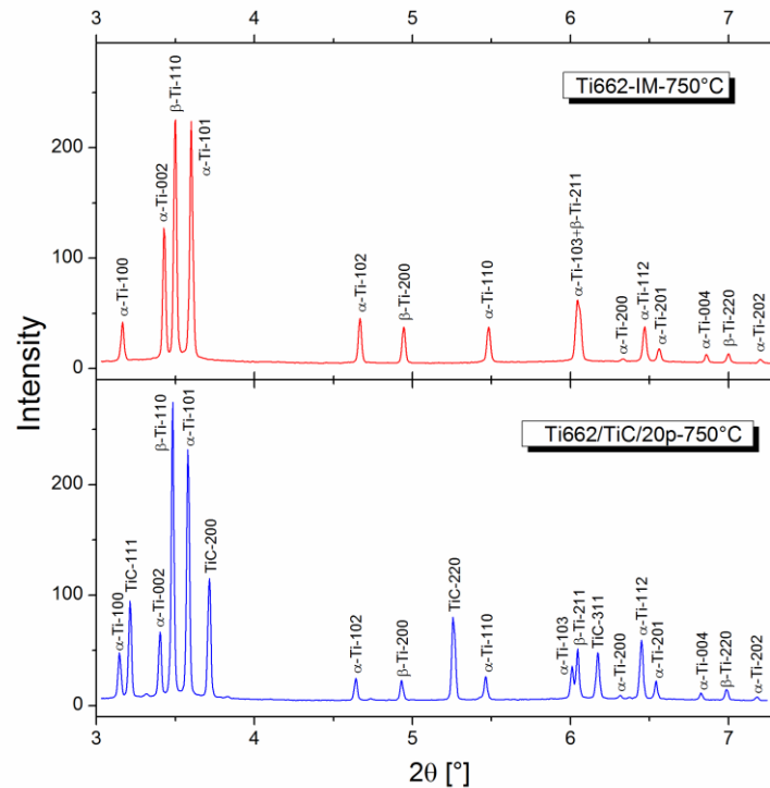
Fig. 3.25. Diffractograms of unreinforced (upper) and reinforced (bottom) Ti662 alloy at 750°C integrated in the axial direction.
