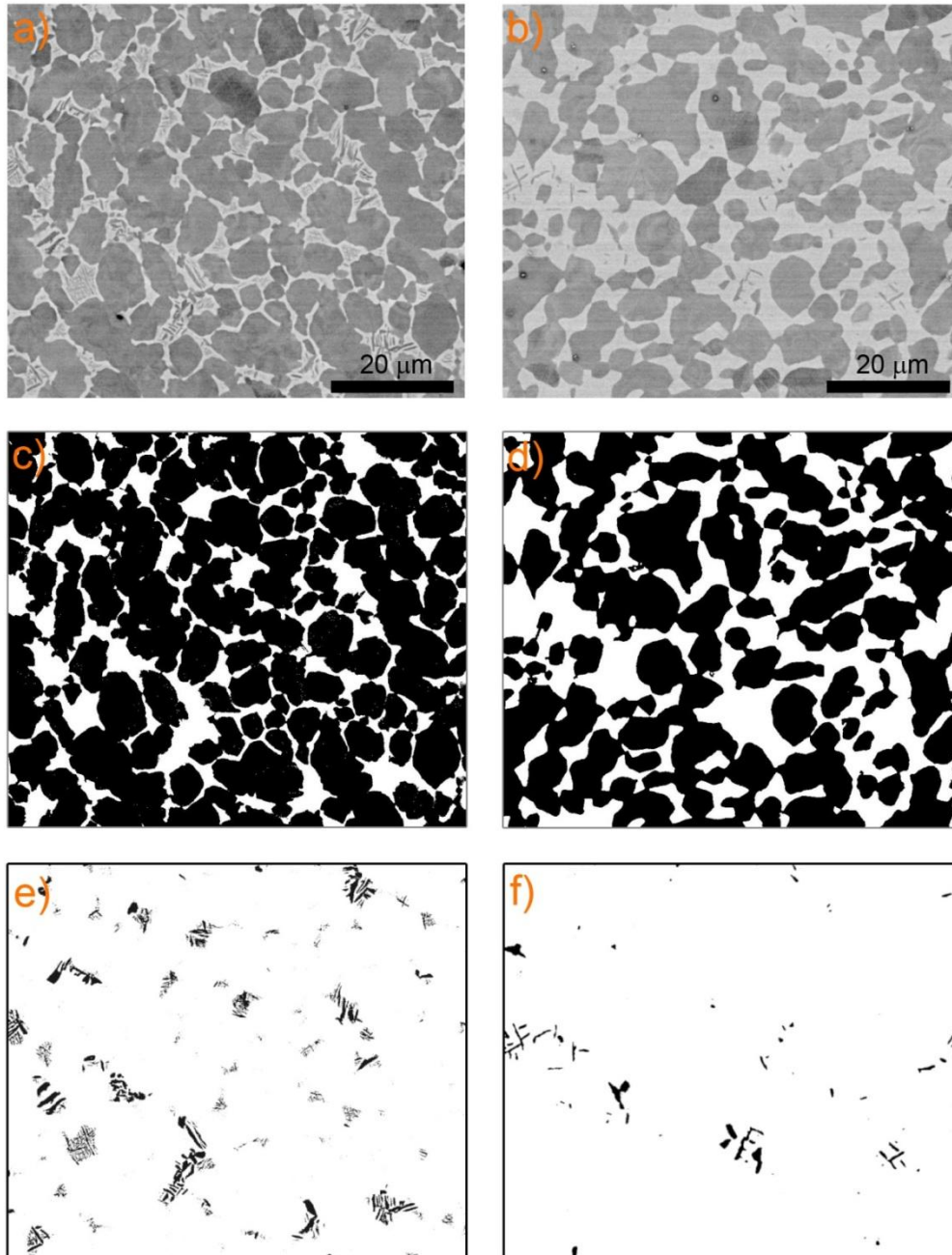
Fig. 4.22. Segmentation of \alpha for the IM alloy: a) and b) show SEM micrographs of the frozen microstructures at 650 and 750°C, respectively. c) and d) show the corresponding segmented \alpha_{\text{primary}} (black) and \beta (white) and e) and f) the segmented \alpha_{\text{secondary}} (black).
