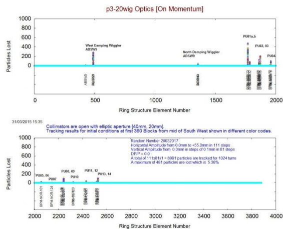
Figure 3: Tracking results for on momentum particles.
