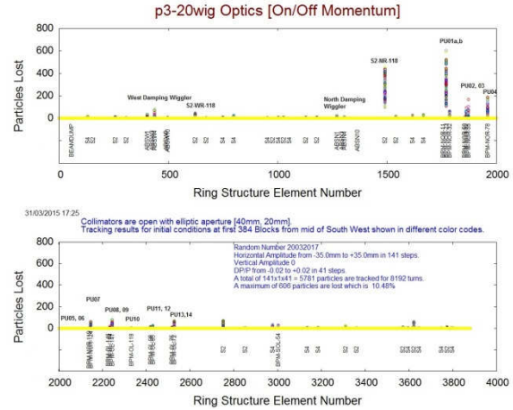
Figure 5: Tracking results for off momentum particles.
