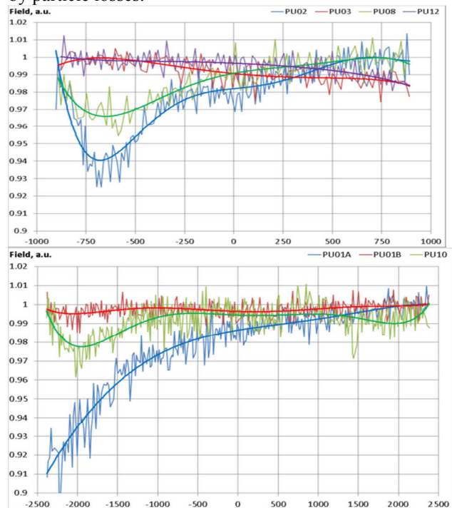
Figure 1: Recently measured longitudinal normalized peak field variation of (a) 2 m devices, (b) 5 m devices installed in PETRA III versus longitudinal position in mm.
