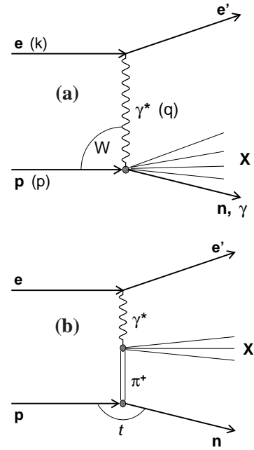
Figure 1: Diagrams for neutron and photon forward production
