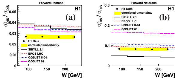
Figure 2: The fraction of DIS events with forward photons (a) and forward neutrons (b) as a function of W . The CR model predictions are compared to the data.
