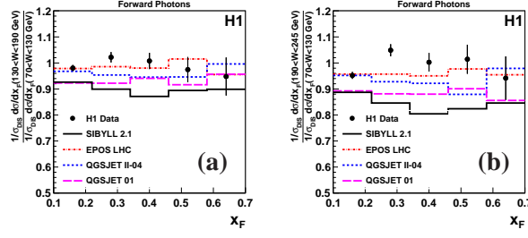
Figure 4: Ratios of normalised cross sections of forward photon production in DIS corresponding to two different W intervals, as a function of x_F : respectively the ratio of the cross section in the 130 < W < 190 GeV (a) and 190 < W < 245 GeV (b) interval to the cross section in the 70 < W < 130 GeV interval. Predictions of the CR models are compared to the data.
