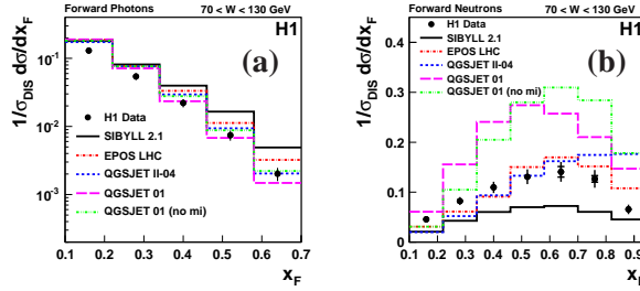
Figure 3: Normalised cross sections of forward photon (a) and forward neutron (b) production in DIS, as a function of x_F in the W -interval 70 – 130 GeV. The CR model predictions are compared to the data.
