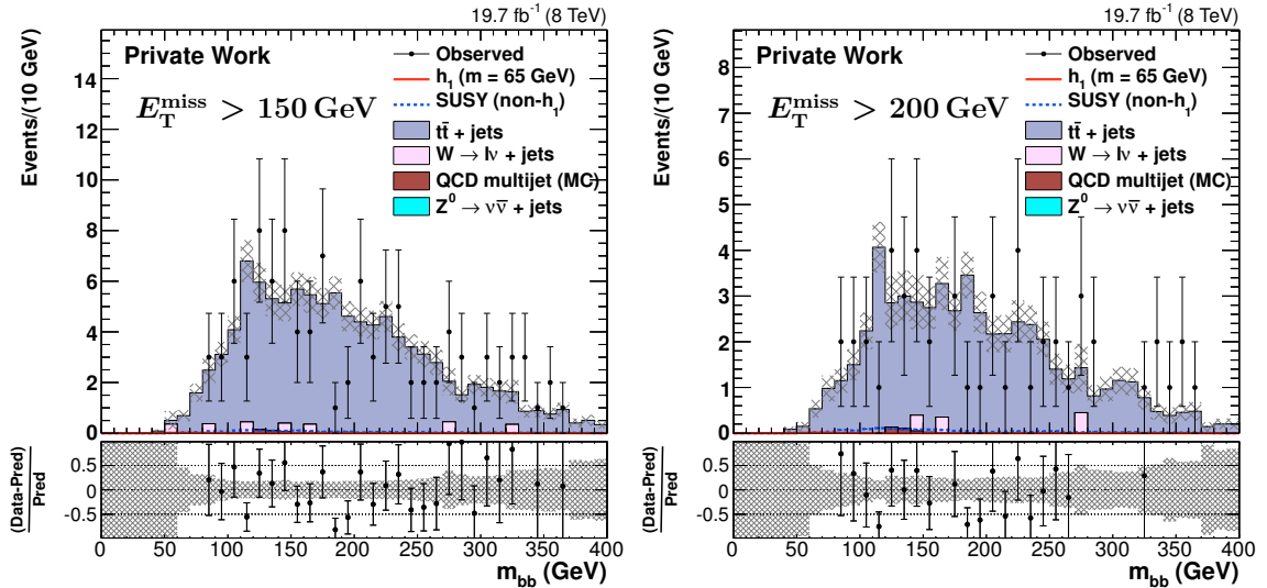
Figure 5.10: Invariant mass of the two selected b-jets in the t\bar{t} control regions based on M_T between the one selected lepton and \vec{E}_T^{\text{miss}} for E_T^{\text{miss}} > 150 GeV (left) and E_T^{\text{miss}} > 200 GeV (right).
