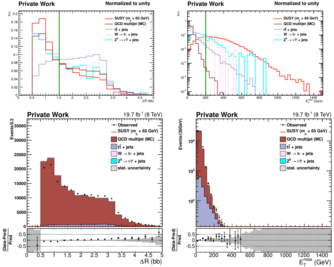
Figure D.4: The \Delta R(b, b) (left) and E_T^{\text{miss}} (right) distributions are shown. The background shape is in agreement with the data distribution. QCD MC is used for illustration purposes only. The analysis uses a data-driven estimate of the QCD background.
