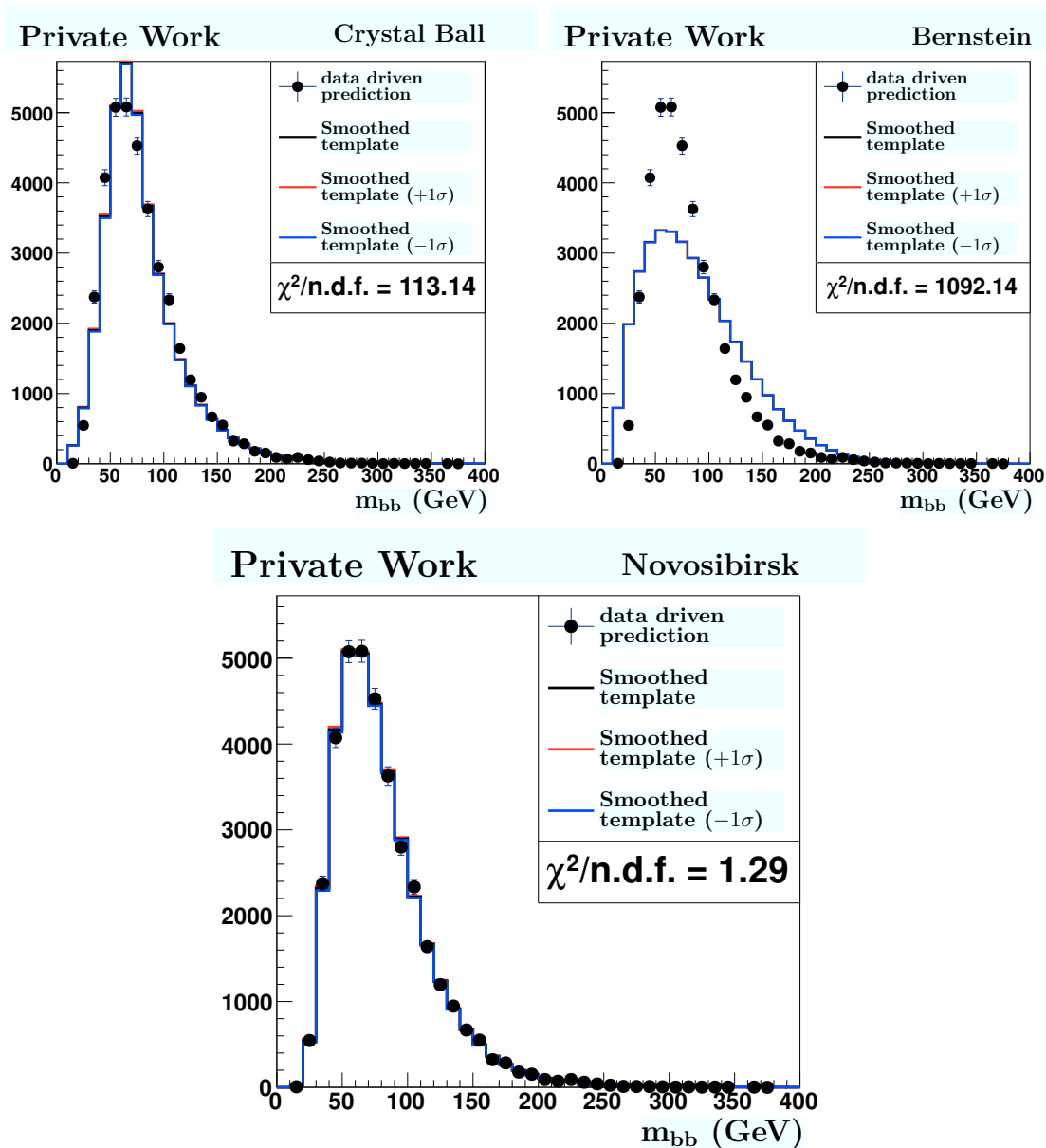
Figure E.2: Fit results of the QCD control region ( E_T^{\text{miss}} \in [0, 50] GeV, veto isolated leptons): Crystal Ball (top left), Bernstein (8th order, top right) and Novosibirsk (bottom). The best fit quality is achieved for the Novosibirsk function.
