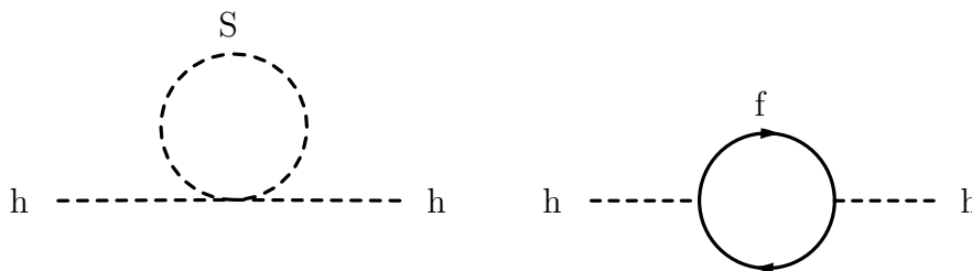
Figure 1.2: One-loop quantum corrections to the Higgs squared mass parameter m_{\text{h}}^2 , due to a scalar S (left), and a Dirac fermion f (right).
