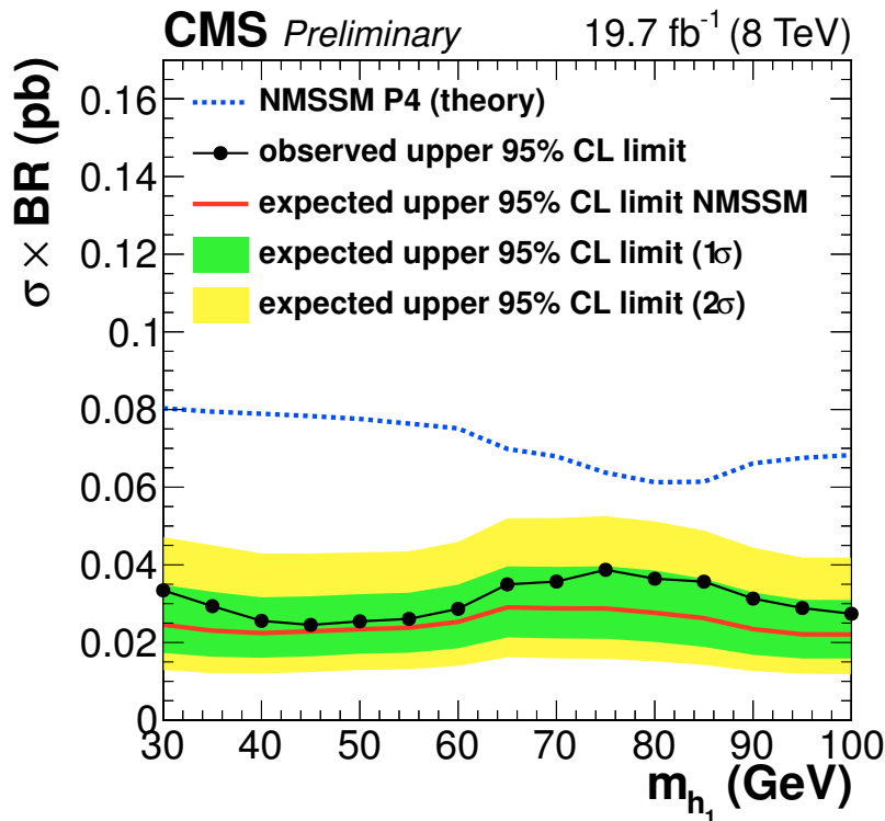
Figure 6.6: Upper limits for the NMSSM cross section times branching fraction into b\bar{b} in comparison to the theoretical expectations from the NMSSM P4 scenario (blue dashed line).
