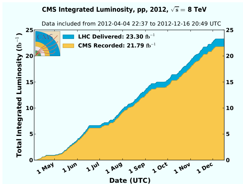
Figure 3.2: Integrated luminosity delivered by the LHC (upper line) and recorded by CMS (lower line) for the data-taking period 2012 [135].
