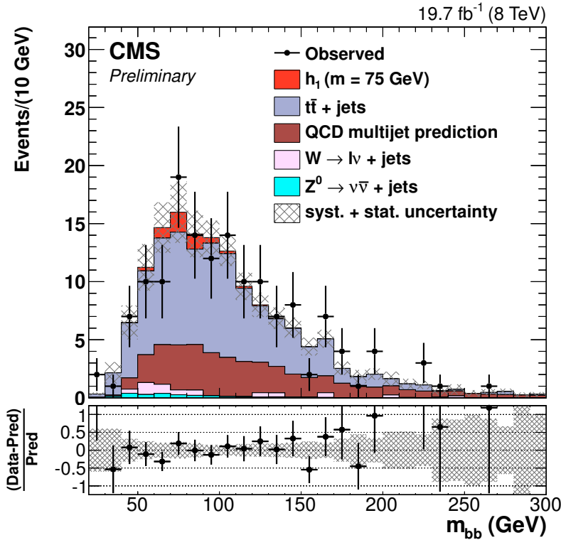
Figure 6.4: Invariant mass of the selected pair of b -tagged jets, where the SM background contributions are stacked. The h_1 template with a mass hypothesis of 75 GeV and the SM-background templates are fitted to the data.
