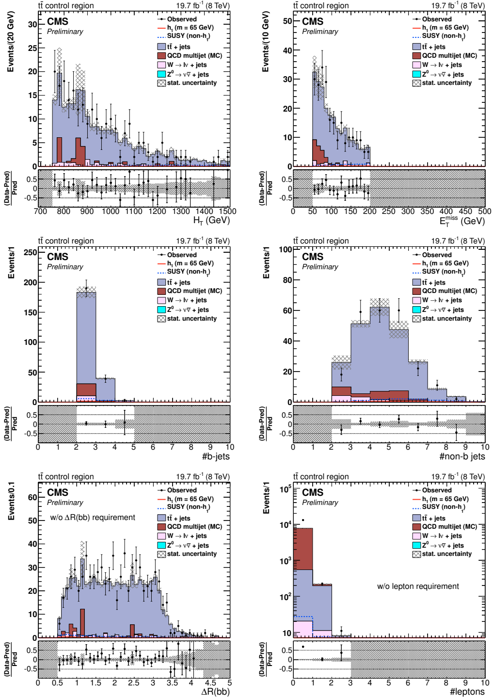
Figure 5.8: Control distributions in the t\bar{t} control region with E_T^{\text{miss}} \in [50, 200] GeV, and \#(\text{isolated leptons}) \geq 1 . The lower left plot has no \Delta R(b,b) requirement and the lower right plot has no requirement on the lepton multiplicity. Good agreement is observed. Note, that the point at \#(\text{leptons}) = 0 in the lower right plot is not part of the t\bar{t} control region and the deviation observed there is attributed to the unreliable QCD-multijet simulation.
