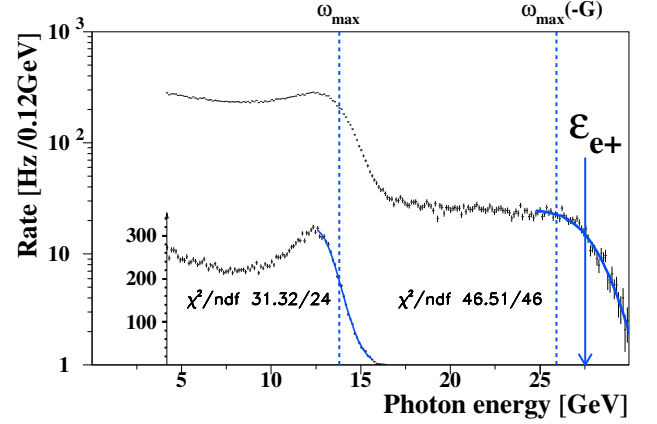
FIG. 3. A similar plot to Fig. 2 for positrons with energy 27.5 GeV. The Compton edge energy for anti-gravitating positrons is indicated by a vertical line \omega_{max}(-G) .
