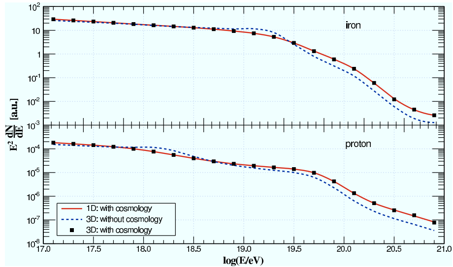
Figure 7.7: Spectra for the 1D simulation (solid line), the 3D without cosmology (dashed line) and the 3D corrected for cosmology (squares) for the pure iron (top) and pure proton (bottom) composition. The spectra are normalized to the total number of events times 100 for iron, and 0.01 for proton.
