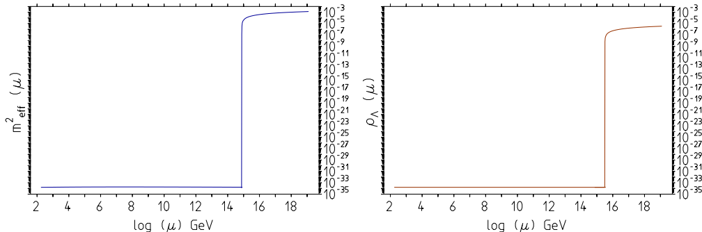
Figure 1: The Higgs potential effective m^2 [left] and the dark energy density [right] in Planck mass units as a function of the energy scale \mu in the SM. Below the matching point \mu_{CC} , where \rho_\Lambda \simeq 1.6 \times 10^{-47} in Planck mass units, we show a scaled up \rho_\Lambda \times 10^{13} value of the present dark energy density \mu_\Lambda^4 with \mu_\Lambda \simeq 0.002 eV.
