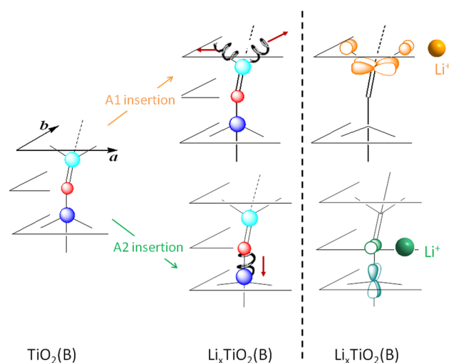
Figure 10. Illustration of the structural changes induced in the local environment of \text{TiO}_5 and \text{TiO}_6 when \text{Li}^+ is inserted in the A1 and A2 sites and the associated electrons fill the antibonding \text{Ti}(d)-\text{O}(2p) orbitals.
