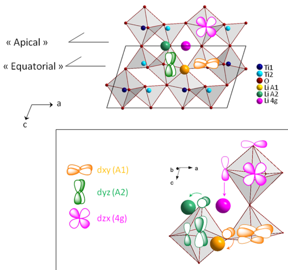
Figure 8. (Top) Superimposition of the d_{xy} (orange), d_{yz} (green), and d_{xz} (pink) orbitals of the TiO n ( n = 5 or 6 ) polyhedra on the unit cell crystal structure of TiO 2 (B). As computed for TiO 2 (B), where the apical and equatorial planes are identified on the left part of the figure. (Bottom) Illustration of the Ti(d)–O(2p) orbital interactions showing the O–Li site activation.
