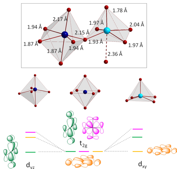
Figure 7. Top: Ti1 (cyan) and Ti2 (blue) local environments as computed for TiO 2 (B). Bottom: Orbital splitting of the t_{2g} orbitals of the regular octahedron ( d_{xy} , d_{yz} , and d_{xz} ) for the pyramidal and pseudo-octahedral environments of Ti1 and Ti2, respectively.
