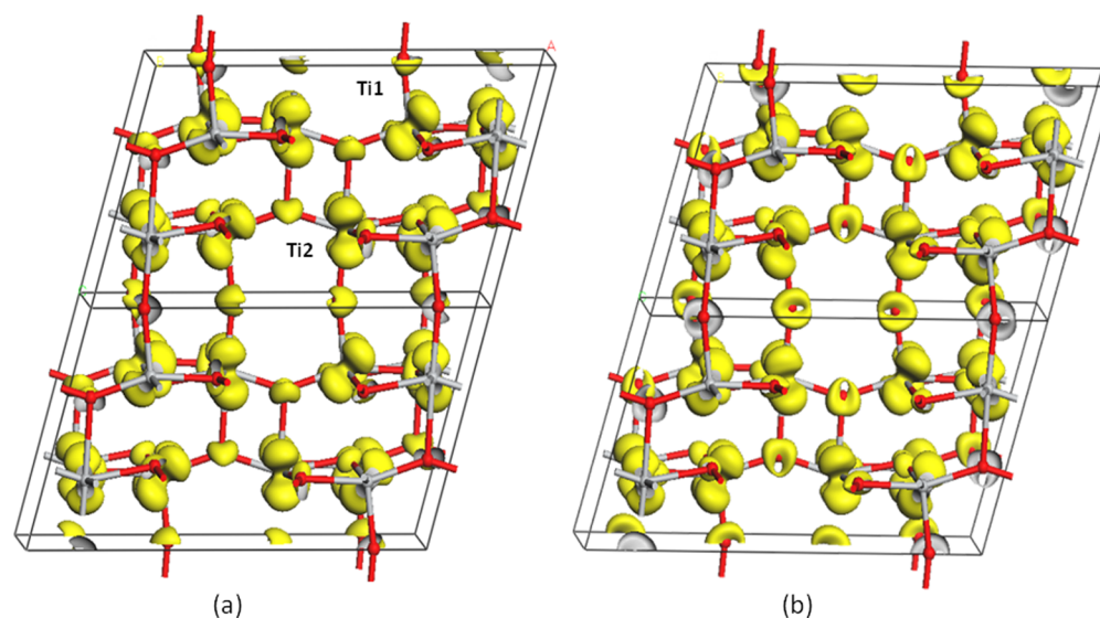
Figure 9. Fukui f^r(r) function computed for \text{TiO}_2(\text{B}) within the DFT+U framework at U = 0 (a) and U = 7 eV (b).
