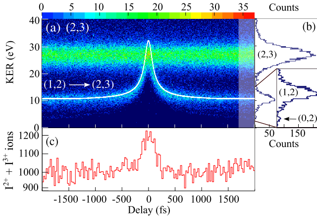
FIG. 2 (color online). (a) KER for all coincident (2,3) ion pairs plotted as a function of the time delay. The classical simulation via the pathway (1,2) \rightarrow (2,3) is superimposed in white. (b) Projection of KERs at large delays (shaded area) onto the KER axis with the inset showing a magnified view of the low-energy region. The charge states belonging to the observed asymptotic KERs are indicated in brackets. (c) Projection of all KERs onto the delay axis.
