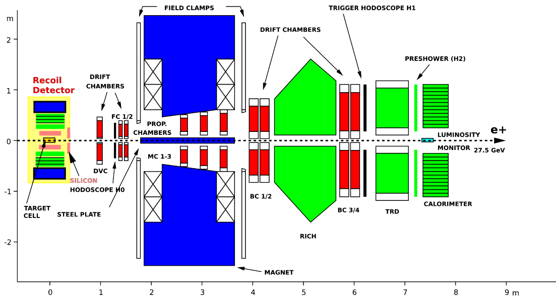
Figure 4.2.2: Schematic side view of the HERMES spectrometer.[2] The lepton beam enters from the left and hits the gas target in the target cell (yellow) inside the recoil detector. The tracking system is colored in red. It consists of DVC, FC, MC and BC. The PID system consisting of RICH, TRD, hodoscope preshower detector and calorimeter is colored in green. The luminosity monitor in light blue can be found after the preshower (H2) at the end of the spectrometer. The yellow underlayed part is the recoil detector added in 2006.
