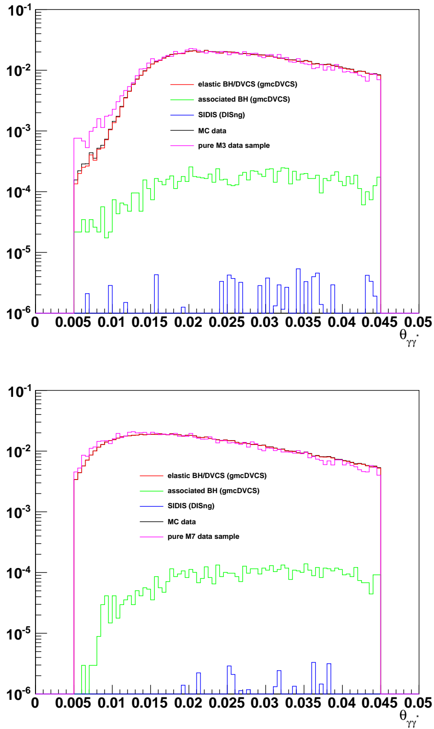
Figure 4.5.9: \theta_{\gamma\gamma^*} distribution of the tracks with best \chi^2_{kin} < 13.7 a in an event for method 3 (top) and method 7 (bottom) in Monte Carlo. For both methods the \theta_{\gamma\gamma^*} distribution is in good agreement between real data and MC.
