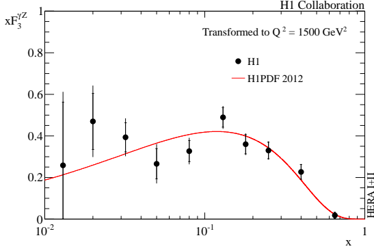
Figure 2. Measurements of x\tilde{F}_3 using the complete H1 data set. The data are compared to a NLO QCD fit.
