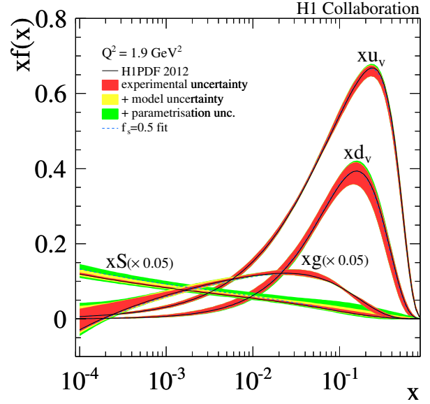
Figure 3. The PDFs determined in the H1PDF2012 NLO QCD fit at the starting scale Q_0^2 = 1.9 \text{ GeV}^2 .
