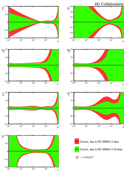
Figure 4. The PDF uncertainties determined in the H1PDF2012 NLO QCD fit obtained from two fits including and excluding the new H1 structure function measurements.
