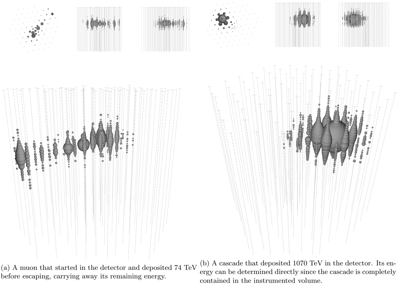
Figure 2: Examples of neutrino event topologies in IceCube from [13]. Each panel is a schematic view of the detector, with each photomultiplier represented by a sphere whose volume is proportional to the collected charge. The smaller upper panels show projections of the detector along its z , x , and y axes, respectively.
