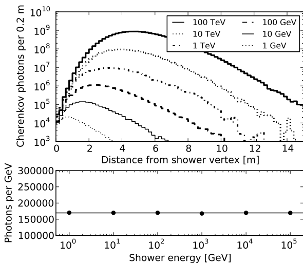
Figure 3: Longitudinal distributions of electromagnetic cascades in ice simulated with GEANT4 [14]. The total light output of the cascade is directly proportional to its energy, while the length of the shower increases only logarithmically with energy. The angular profile of light emission is nearly identical across the entire energy range [3]. The range in positions of the shower maximum (between 1 and 5 meters from the vertex here) is small enough that the showers can be considered pointlike on the scale of IceCube instrumentation. Hadronic showers have nearly identical properties when viewed with IceCube [3].
