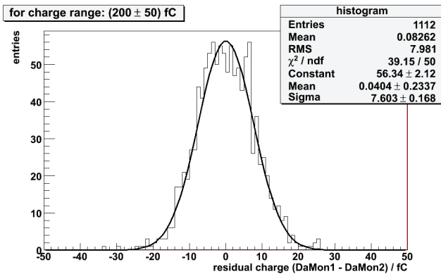
Figure 6: Residuals between charge measurement of both DaMon channels for a charge around 200 fC with a Gaussian fit.
