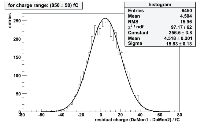
Figure 7: Residuals between charge measurement of both DaMon channels for a charge around 850 fC with a Gaussian fit.
