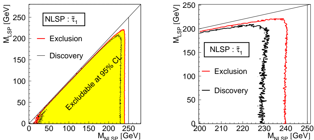
Figure 4: Discovery reach for a \tilde{\tau}_1 NLSP after collecting 500 \text{ fb}^{-1} at \sqrt{s} = 500 GeV. Left: full scale, Right: zoom of the region close to the kinematic limit.
