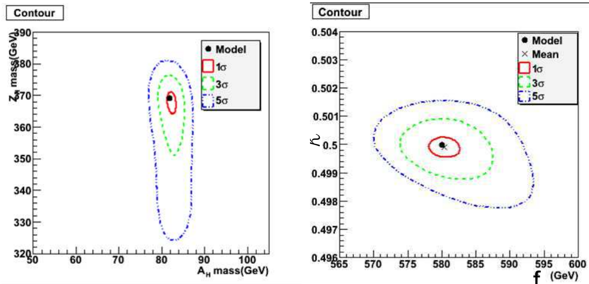
Figure 10: Accuracy of T-odd particle mass (left) and model parameter (right) determination for a representative benchmark point in the parameter space of the Littlest Higgs model with T-parity. From [63].
