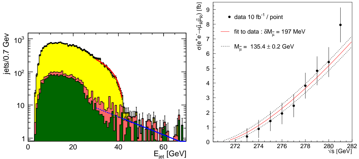
Figure 6: Left: \tilde{\tau}_1 spectrum (yellow) and background (SM: red, other SUSY: green), with end-point fit. From Ref. [40]. Right: Threshold scan at the e^+e^- \rightarrow \tilde{\mu}_R\tilde{\mu}_R threshold. From Ref. [41]
