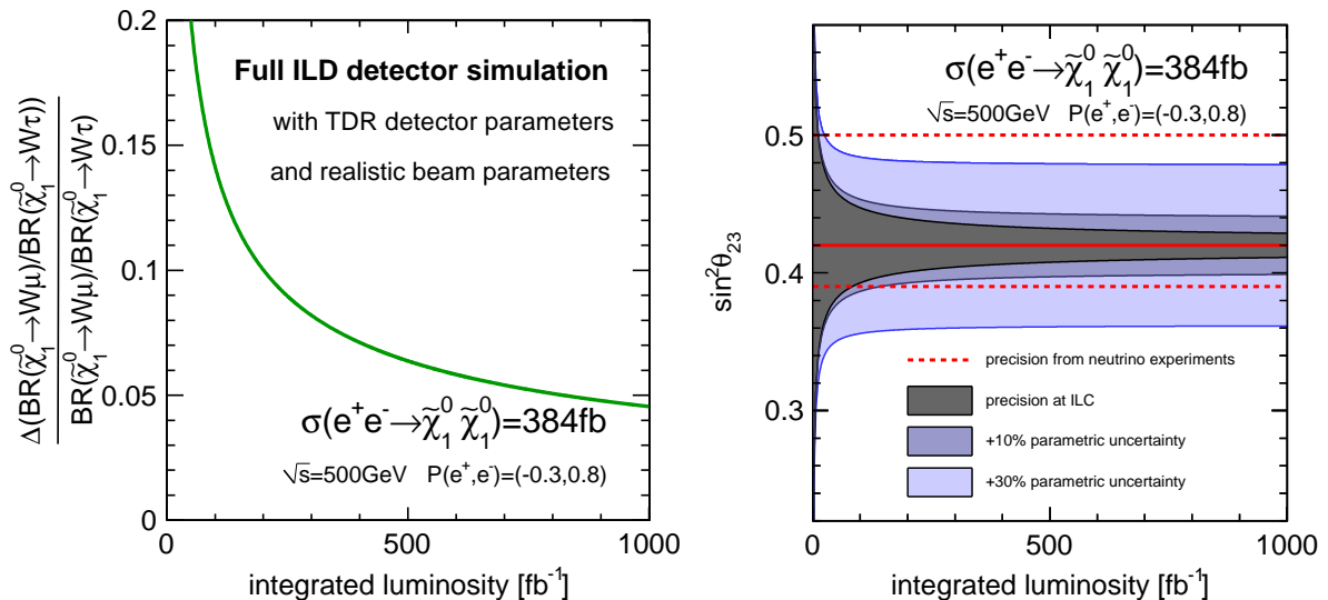
Figure 8: Left: Experimental precision on BR(\tilde{\chi}_1^0 \rightarrow W\mu)/BR(\tilde{\chi}_1^0 \rightarrow W\tau) as a function of the integrated luminosity for the simulated benchmark point. Right: Derived uncertainty on the atmospheric neutrino mixing angle \sin^2 \theta_{23} , including the additional parametric uncertainty due to limited knowledge of other SUSY parameters.
