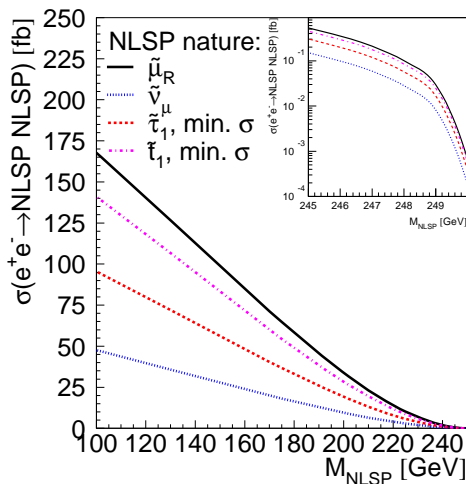
Figure 2: NLSP production cross sections as a function of M_{\text{NLSP}} at \sqrt{s} = 500 \text{ GeV} (best beam polarization) for a few NLSP hypotheses. The insert shows the last few GeV before the kinematic limit, on a log scale.
