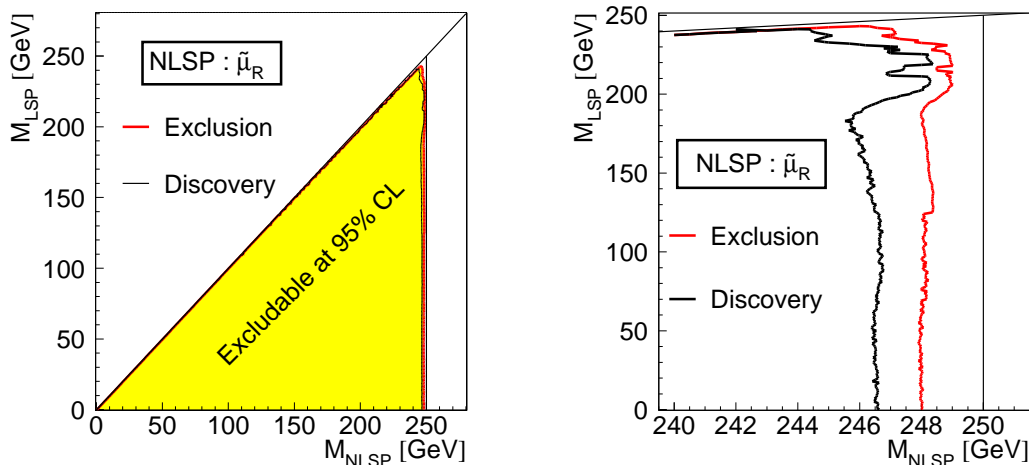
Figure 3: Discovery reach for a \tilde{\mu}_R NLSP after collecting 500 \text{ fb}^{-1} at \sqrt{s} = 500 GeV. Left: full scale, Right: zoom to last few GeV before the kinematic limit.
