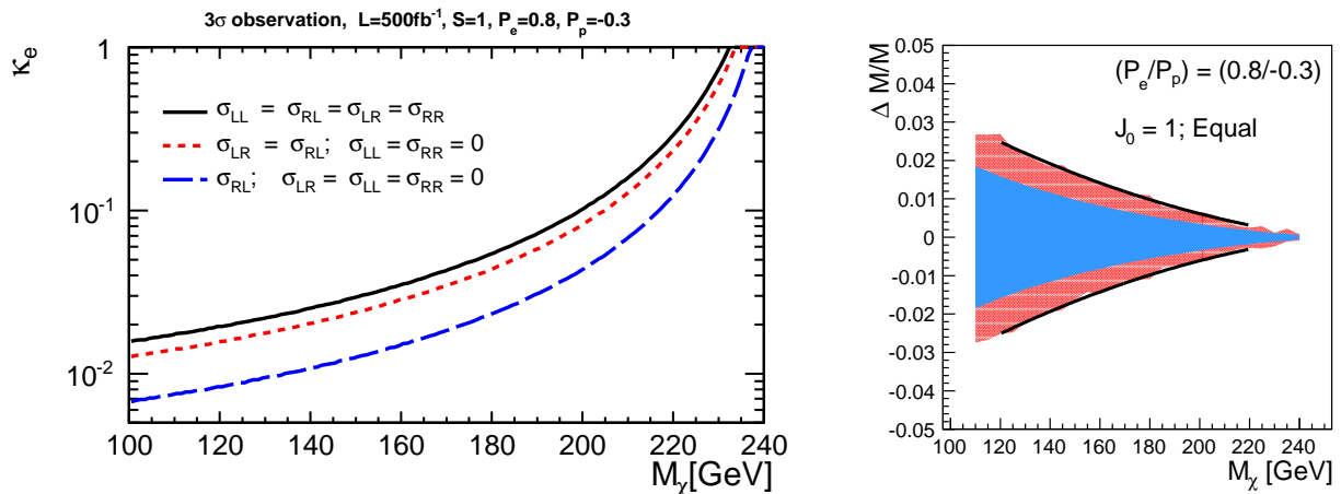
Figure 9: Left: Observational reach ( 3\sigma ) of the ILC for a Spin-1 WIMP in terms of WIMP mass and \kappa_e for three different chiralities of the WIMP-fermion couplings [53] (Note: At WIMP masses lower than \sim 150 GeV, not all assumptions in the relation between the WIMP annihilation and e^+e^- production cross-sections are fully valid anymore. Signals of low mass WIMPs could still easily be observed, but the interpretation of \kappa_e becomes somewhat less straight forward, since for too low masses the WIMP production is not non-relativistic anymore). Right: Experimental statistical (red) and systematic (blue) precision of the mass reconstruction as a function of the WIMP mass. From Ref. [54].
