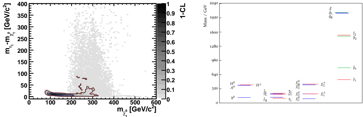
Figure 5: Left: Likelihood of a constrained MSSM fit to pre-LHC experimental data in the \Delta M(\tilde{\tau}, \tilde{\chi}_1^0) - M_{\tilde{\chi}_1^0} plane. The series of example points discussed here have \Delta M(\tilde{\tau}, \tilde{\chi}_1^0) - M_{\tilde{\chi}_1^0} = 10 GeV, right on the strip of highest likelihood, from Ref. [35]. Right: Spectrum of one of the example scenarios, from Ref. [37]
