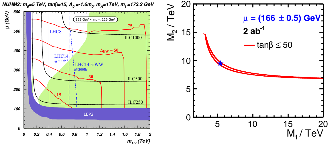
Figure 1: Left: Contours of fine-tuning \Delta_{EW} = 15, 30, 50, and 75 in the m_{1/2} vs. \mu plane for the RNS model with parameters as shown (from Ref. [27]). The blue vertical lines show the current reach of LHC8 and the projected reach of LHC14 with 300 \text{ fb}^{-1} via gluino pair searches (dashed line) and same-sign dibosons (dot-dashed). The reach of ILC with \sqrt{s} = 250, 500 and 1000 TeV is also shown. The green-shaded region has a thermal Higgsino relic abundance \Omega_{\tilde{h}} h^2 \leq 0.12 . Right: Parameter determination in the M_2 vs M_1 plane in the benchmark Higgsino scenario. The star indicates the input values of M_2 and M_1 , the \Delta\chi^2 = 1 contour of a fit to expected ILC measurements is displayed in red. From the same fit, \mu is obtained with sub-GeV precision. From Ref. [32].
