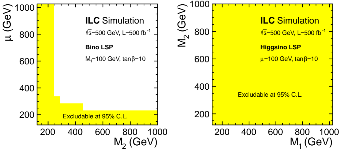
Figure 7: Exclusion reach for electroweakinos at the ILC studied with fast simulation. Left: the case of Bino LSP. Right: the case of Higgsino LSP. The shaded region (yellow) is the expected exclusion reach at 95% confidence level.
