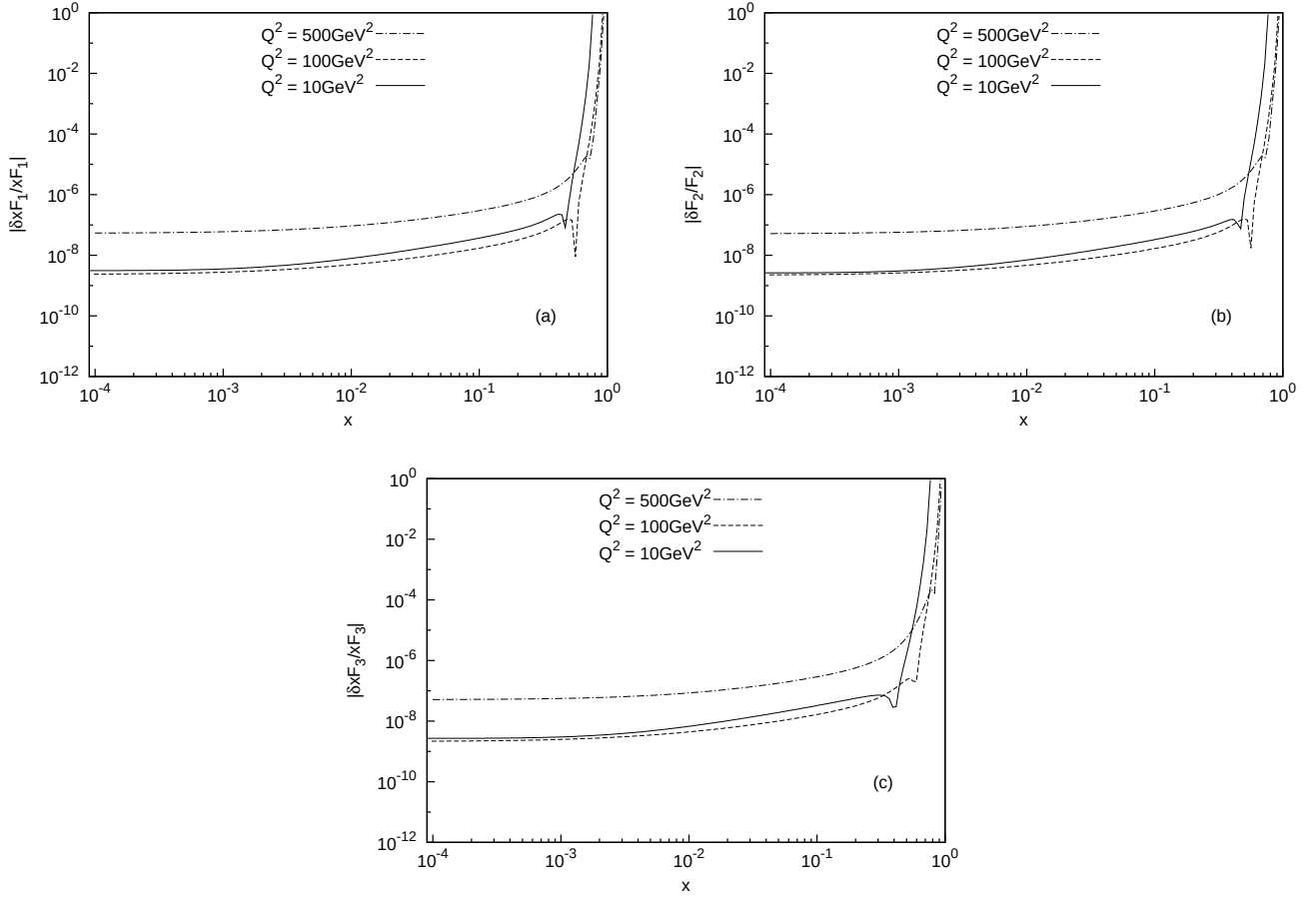
Figure 7: Relative accuracy of the charged current structure functions F_{i,c}^{W+} to O(\alpha_s) at Q^2 = 10, 100, 500 \text{ GeV}^2 , comparing the implementation in Mellin- and z -space. Here both for f_{1,2}(\lambda, N) the analytic representation (514, 515) and their recurrences were used; from [134].
