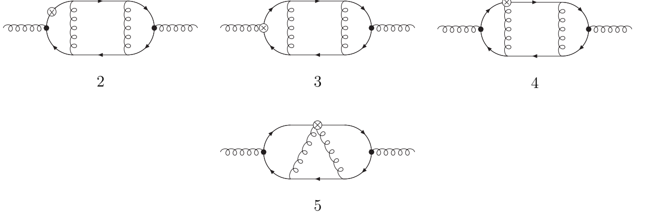
Figure 4: Diagrams with 6 fermion propagators
