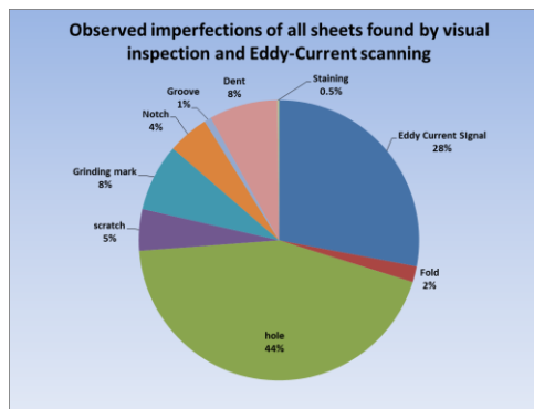
Figure 2: Observed imperfections found by Eddy-Current testing and visual inspection in total.
