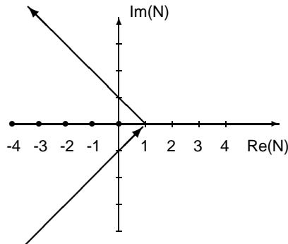
Fig. 2 Path of the contour integral (112).
