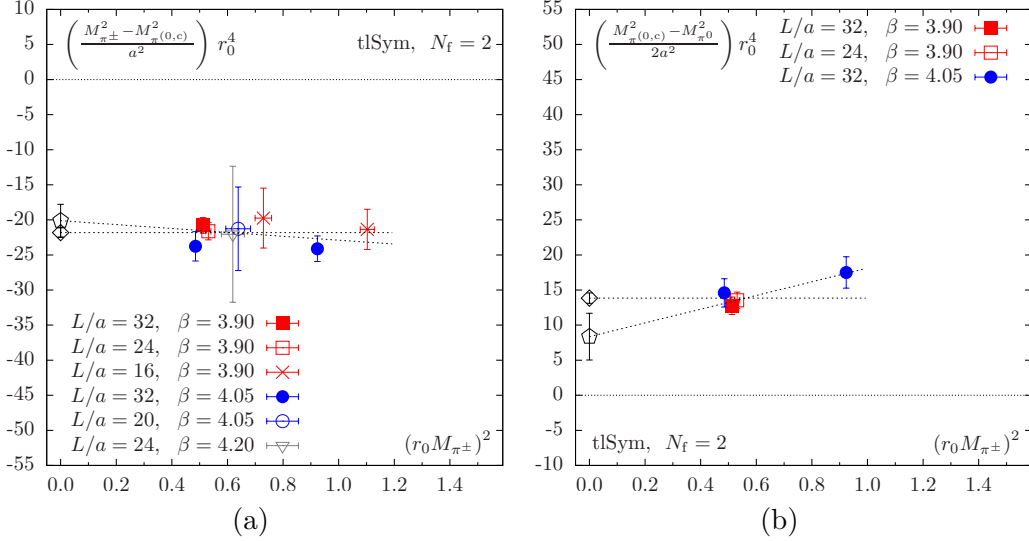
Fig. 3. Determination of the mass-splittings (a) (M_{\pi^\pm}^2 - M_{\pi^{(0,c)}}^2)/a^2 in eq. (6) and (b) (M_{\pi^{(0,c)}}^2 - M_{\pi^0}^2)/2a^2 in eq. (7) as a function of M_{\pi^\pm}^2 . These quantities are in units of the chirally extrapolated Sommer scale r_0 . The mass-splittings are directly related to the Wilson LECs W'_8 and W'_6 . The lattice setup with the tree-level Symanzik improved (tlSym) gauge action and N_f = 2 flavours of Wilson twisted mass fermions is considered. Filled and empty symbols signal a change in the lattice size.
