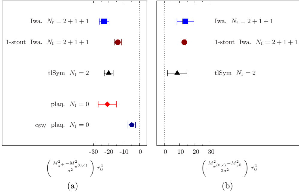
Fig. 5. Comparison of the values of the mass-splittings (a) (M_{\pi^\pm}^2 - M_{\pi^{(0,c)}}^2)/a^2 and (b) (M_{\pi^{(0,c)}}^2 - M_{\pi^0}^2)/2a^2 from different lattice setups (see text for details).
