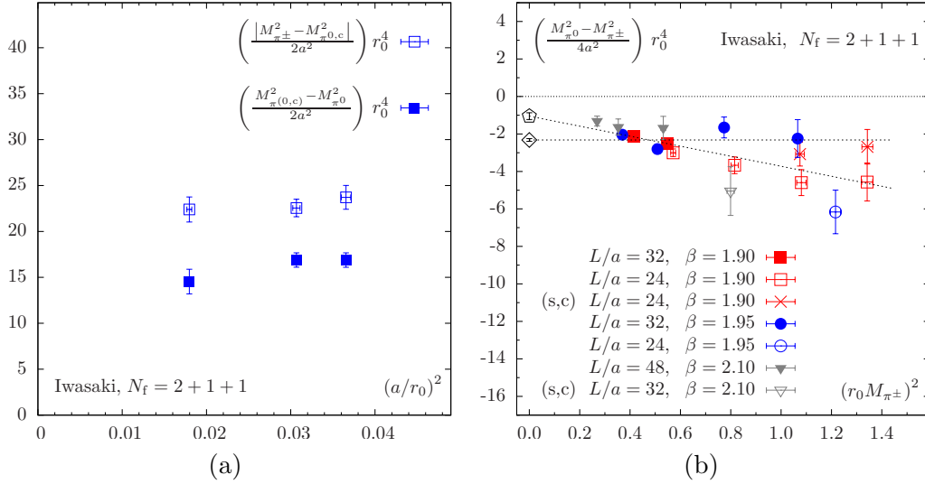
Fig. 2. (a) Lattice spacing dependence of the mass-splittings |M_{\pi^\pm}^2 - M_{\pi^{0,c}}^2|/a^2 – empty symbols – and (M_{\pi^{0,c}}^2 - M_{\pi^0}^2)/2a^2 – filled symbols – at a reference mass (M_{\pi^\pm} r_0)^2 \approx 0.55 . For a better visibility, the absolute value of the mass splitting is considered in the case of the empty symbols. (b) Pion mass-splitting, (M_{\pi^0}^2 - M_{\pi^\pm}^2)/a^2 , normalised according to eq. (9) in order to relate it to the combination of Wilson LECs c_2 . The chiral extrapolation using a constant and a linear fit in M_{\pi^\pm}^2 is also shown. The lattice setup with the Iwasaki gauge action and N_f = 2 + 1 + 1 flavours of Wilson twisted mass fermions is considered.
