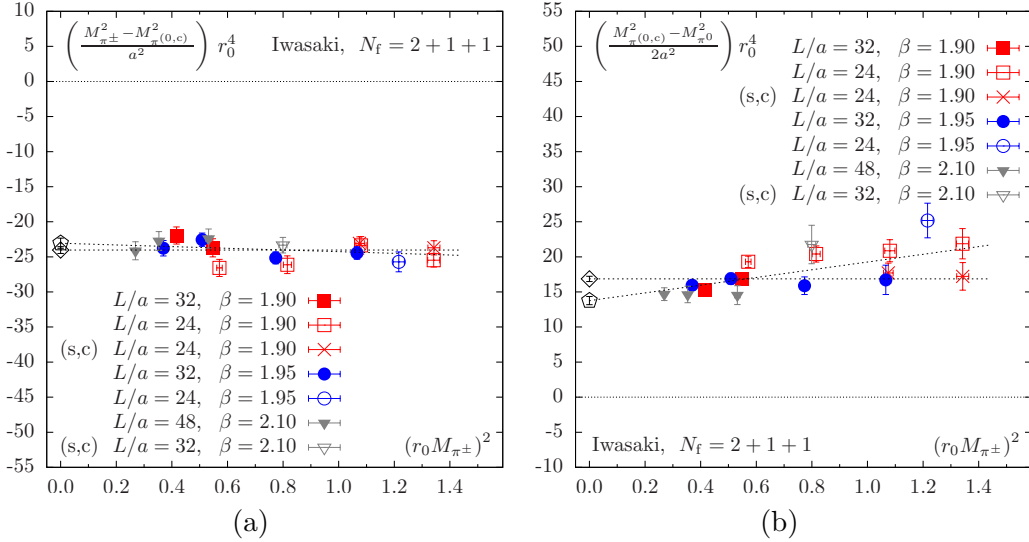
Fig. 1. Determination of the mass-splittings (a) (M_{\pi^\pm}^2 - M_{\pi^{(0,c)}}^2)/a^2 in eq. (6) and (b) (M_{\pi^{(0,c)}}^2 - M_{\pi^0}^2)/2a^2 in eq. (7) as a function of M_{\pi^\pm}^2 . These quantities are in units of the chirally extrapolated Sommer scale r_0 . The mass-splittings are directly related to the Wilson LECs W'_8 and W'_6 . The lattice setup with the Iwasaki gauge action and N_f = 2 + 1 + 1 flavours of Wilson twisted mass fermions is considered. Filled and empty symbols signal a change in the lattice size. The label “(s,c)” in the legend indicates the effect of changing the values of the strange and charm quark masses in the sea. The mass-splittings illustrated in these figures assess the size of O(a^2) discretisation effects. Hence, any lattice spacing dependence in these quantities points to residual higher order discretisation effects. The results of a chiral extrapolation from a constant and a linear fit in M_{\pi^\pm}^2 are shown. The deviation between the two extrapolated values is included in the systematic error analysis.
