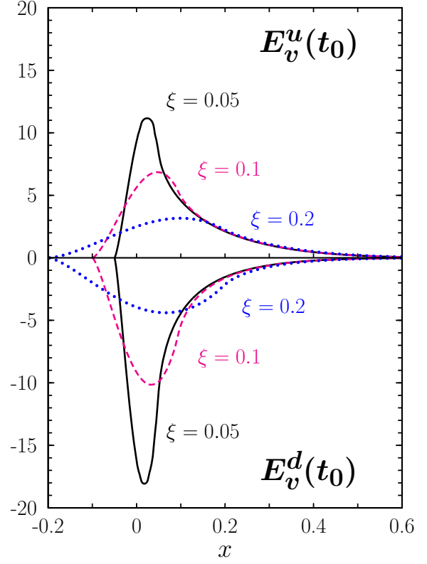
Figure 27: The valence GPD E_v^q at the scale \mu = 2 \text{ GeV} for selected values of \xi . We set -t to its minimum value -t_0 = 4\xi^2 m^2 / (1-\xi^2) that can be achieved in a physical process at given \xi .
